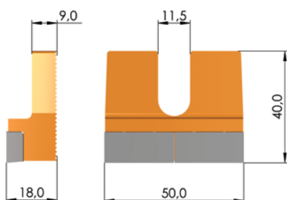
SCRAPER 50x40x18 part-no. 14010013
