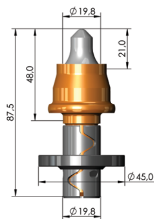
RM3-T8 XL part-no. 11032147
