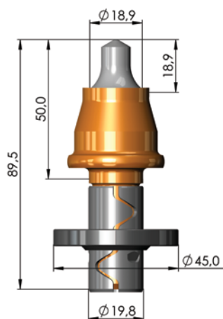
RM3-T6 XL part-no. 11032500 RM3-TN6 XL WITH EXTRACTOR GROOVE part-no. 11032501
