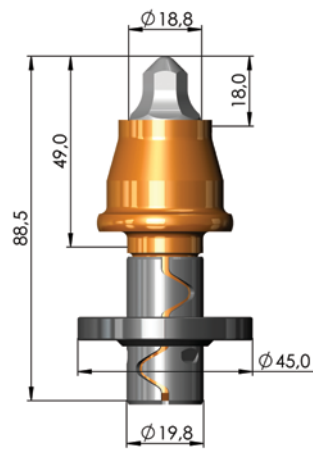
RM3-T9 part-no. 11032133 RM3-TN9 WITH EXTRACTOR GROOVE part-no. 11032137
