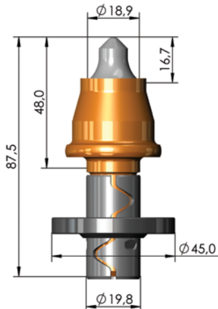
RM3-T6 part-no. 11032330 RM3-TN6 WITH EXTRACTOR GROOVE part-no. 11032141
