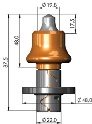
RM3-22/B7 HD part-no. 11032558
