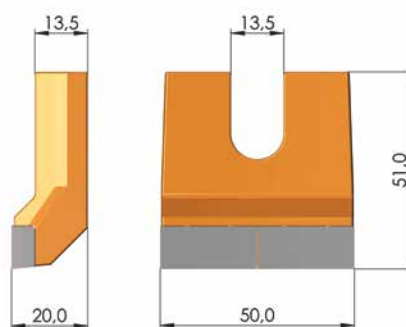
SCRAPER 50x51x20 part-no. 14010001
